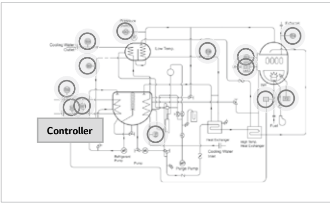
Piping Diagram
