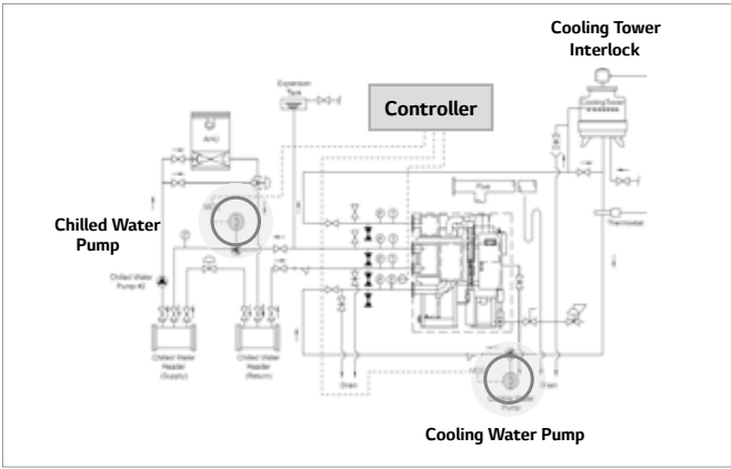
Equip. Facility Diagram
