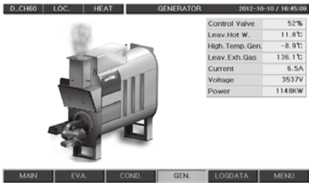
High temperature generator
