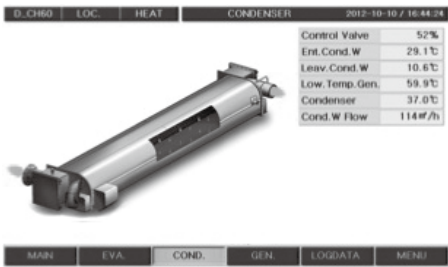
Low temperature generator
