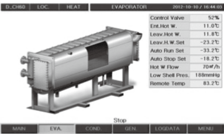
Evaporator & absorber
